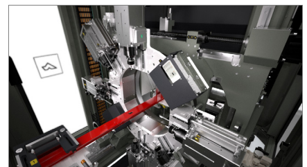
Milling unit 02
